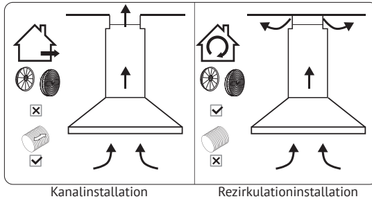
Kanalinstallation
